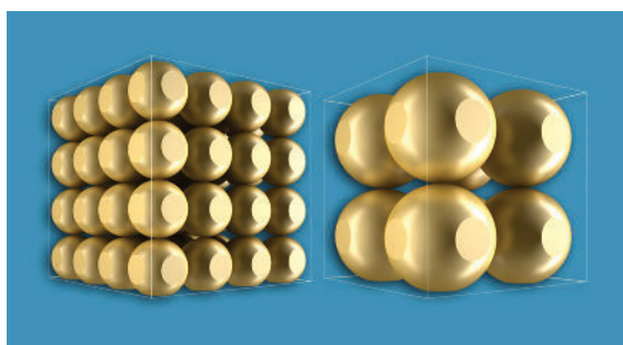
Figure 9. For a given volume, the radius of the fat particles is inversely proportional to its contact surface. Reducing the particle size increases the contact surface with the surrounding capillaries.
